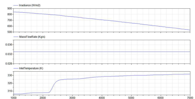
Figure 9. Case C Irradiance, mass flow rate, and inlet temperature profiles.
