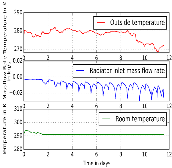
Figure 7. PID Controller flow regulation (middle figure) and the room temperature maintained as a result (bottom figure).
